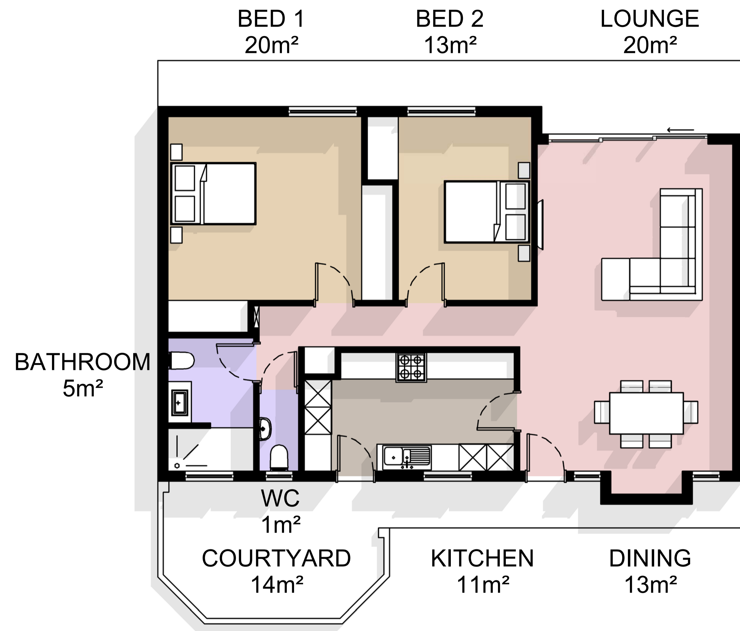
2 BEDROOM COTTAGE- TYPE B
